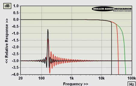
ABOVE: Time (linear phase filter, black; minimum phase filter, red) and magnitude responses at 48kHz (black), 96kFs (red) and 192kFs (green)
