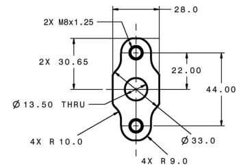
Oil Outlet
