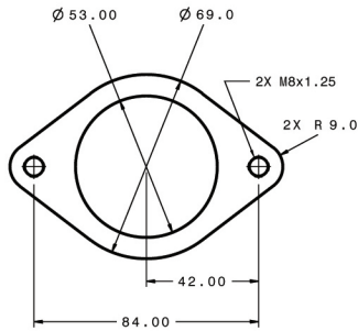
Compressor Inlet
