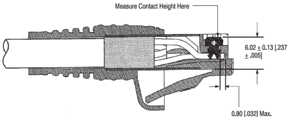
Figure 15: Connector Termination Requirements
