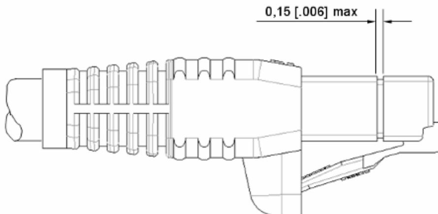
Figure 16: Connector Termination Requirements
